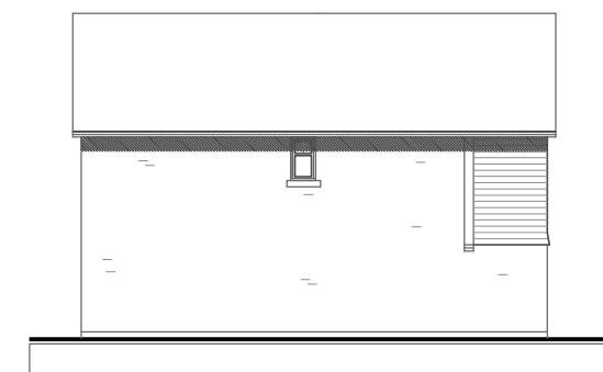
9. SIDE ELEVATION - South
