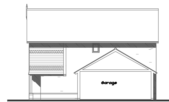
7. (6) SIDE ELEVATION - East (West Elevation plot 6 - handed)
