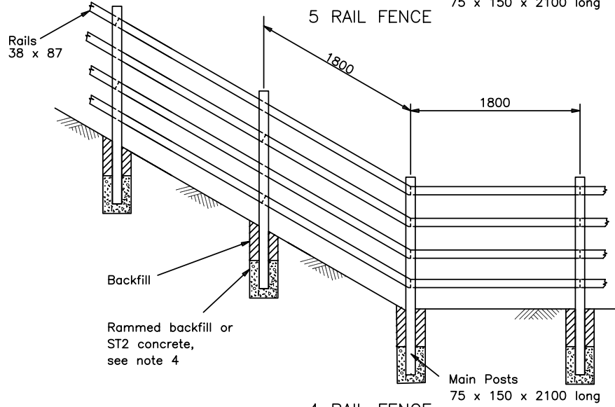
4 RAIL FENCE
