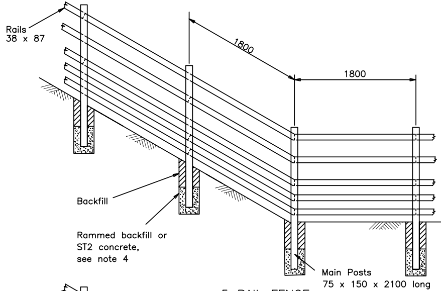
5 RAIL FENCE
