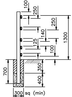
SECTION THROUGH Q OF MAIN POSTS
