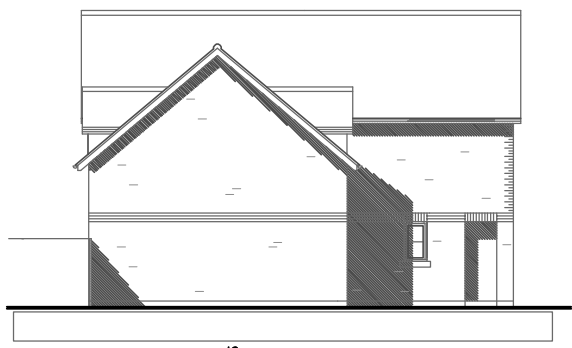
SIDE ELEVATION - North
