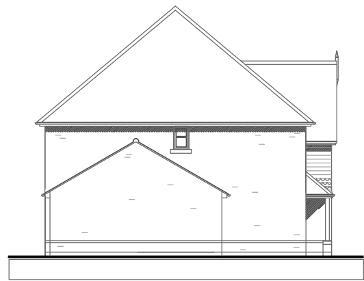
SIDE ELEVATION - East
