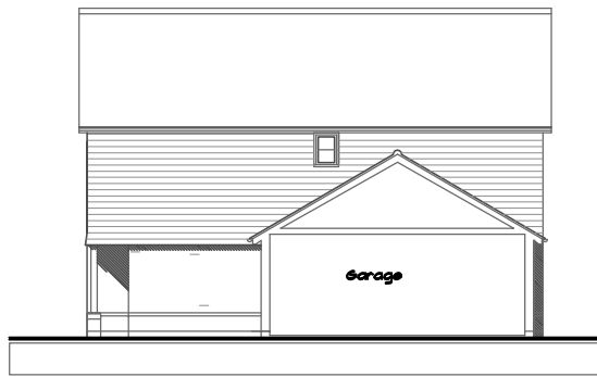
SIDE ELEVATION - West Side Elevation plot 14 similar but handed
