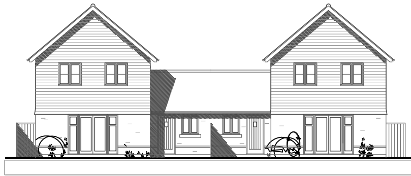
REAR ELEVATION - North
