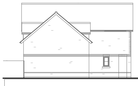
11. SIDE ELEVATION - East
