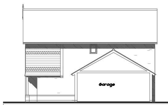
7. (6) SIDE ELEVATION - East (West Elevation plot 6 - handed)
