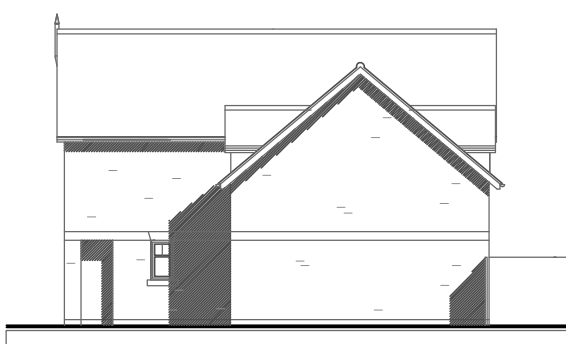
8 & 10 SIDE ELEVATION - North
