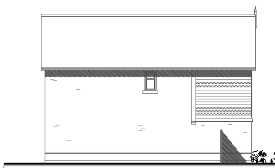
7. (6) SIDE ELEVATION - West (East elevation plot 6 - handed)
