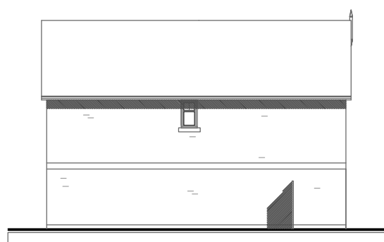
8 & 10 SIDE ELEVATION - South
