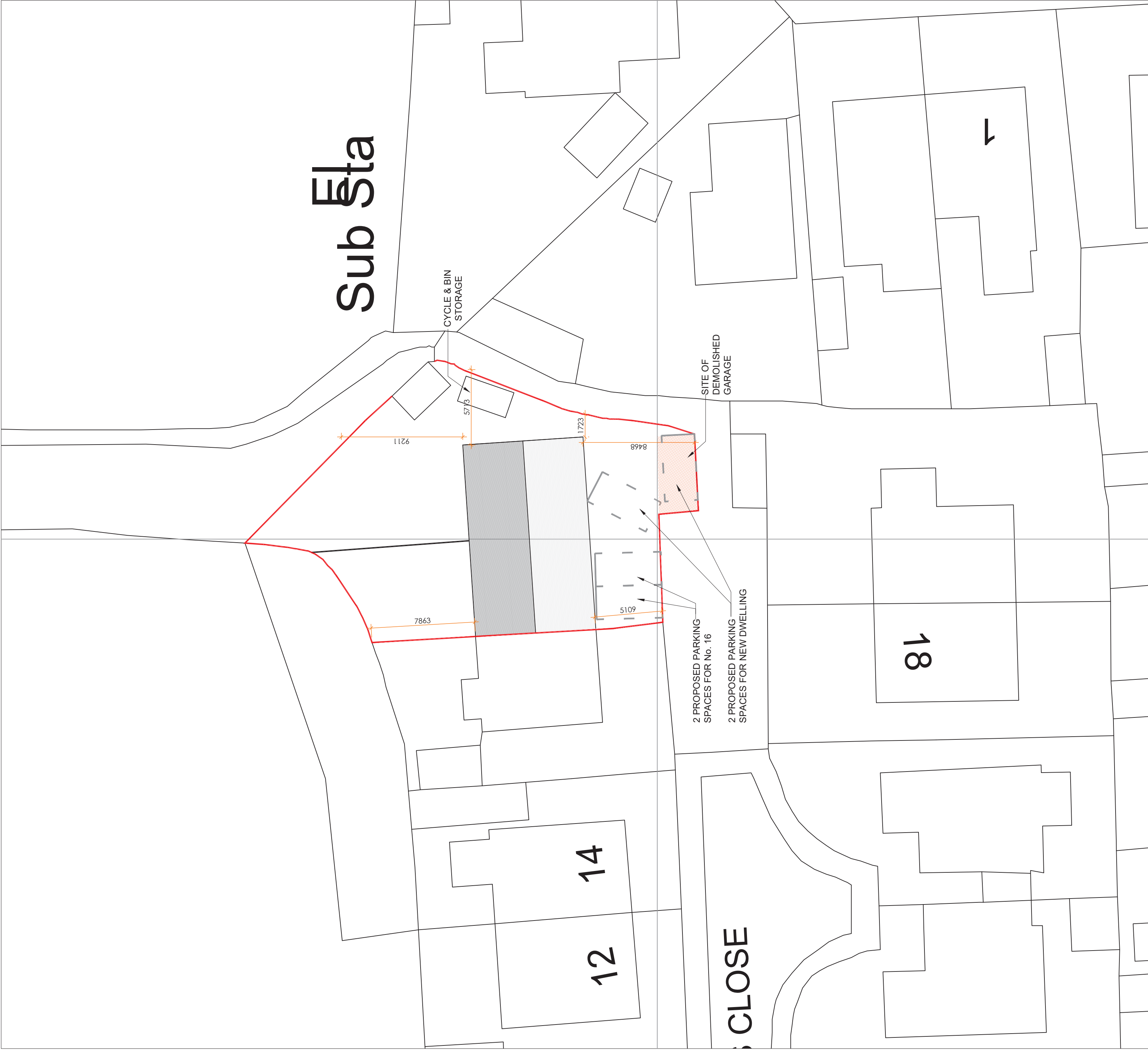
BLOCK PLAN (SHOWING PROPOSED) Scale 1:200
