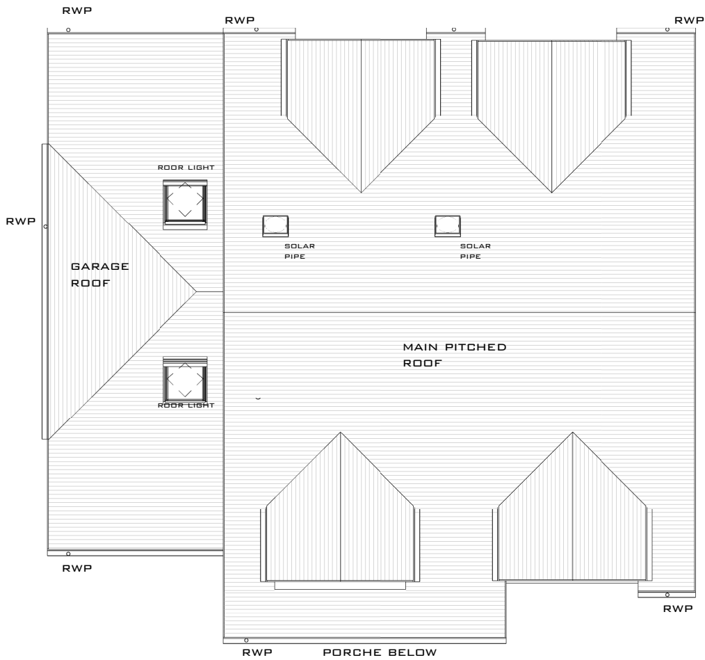
Roof Plan
