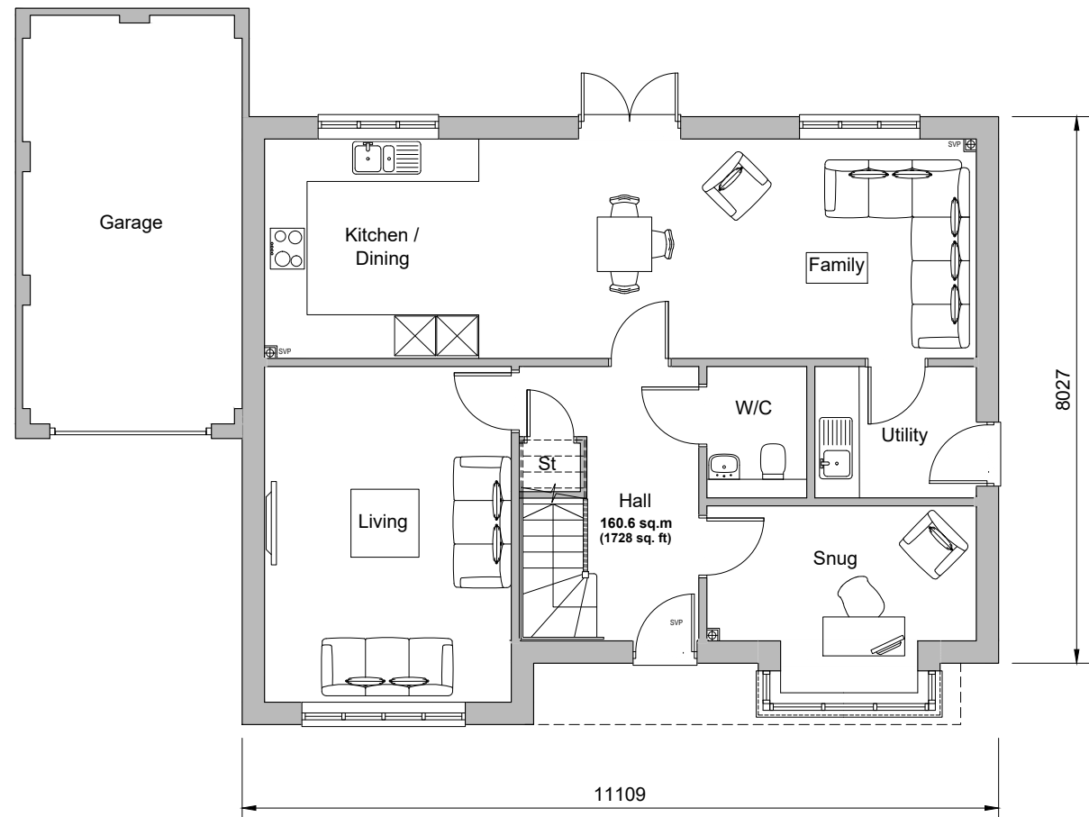
Ground Floor Plan Plot 327
