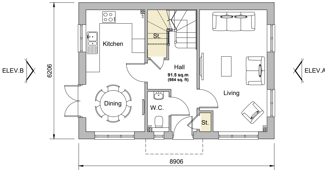
Ground Floor Plan Plots 180
