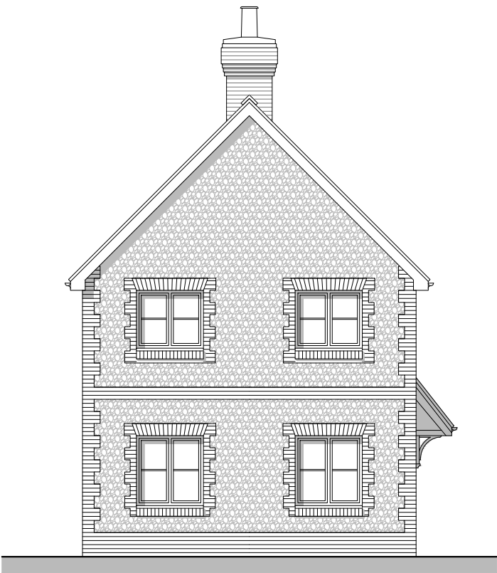
Side Elevation B
