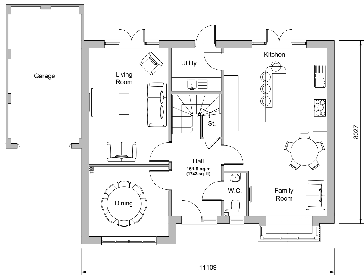
Ground Floor Plan Plot 218
