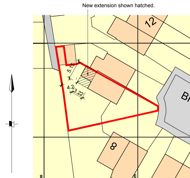
Proposed Site / block plan 1:500 @ A3
