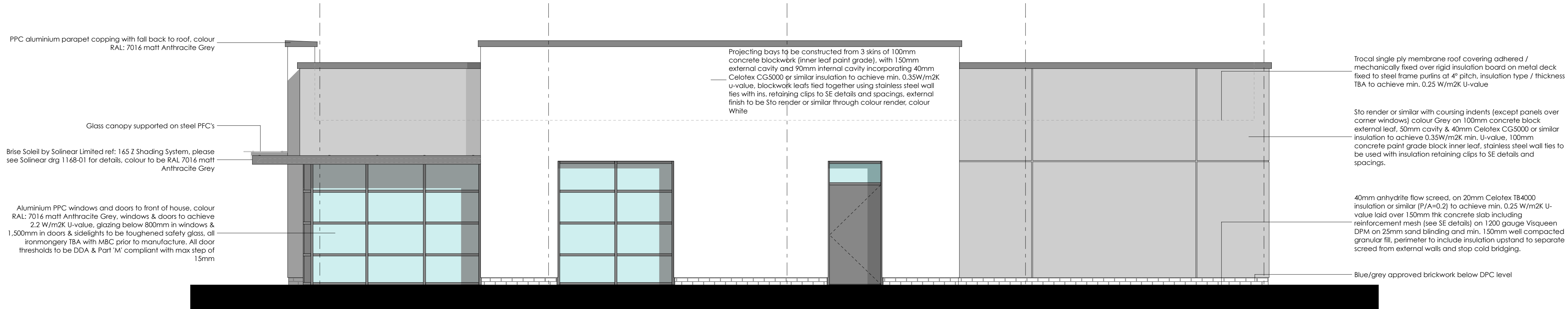
Elevations 1:50
