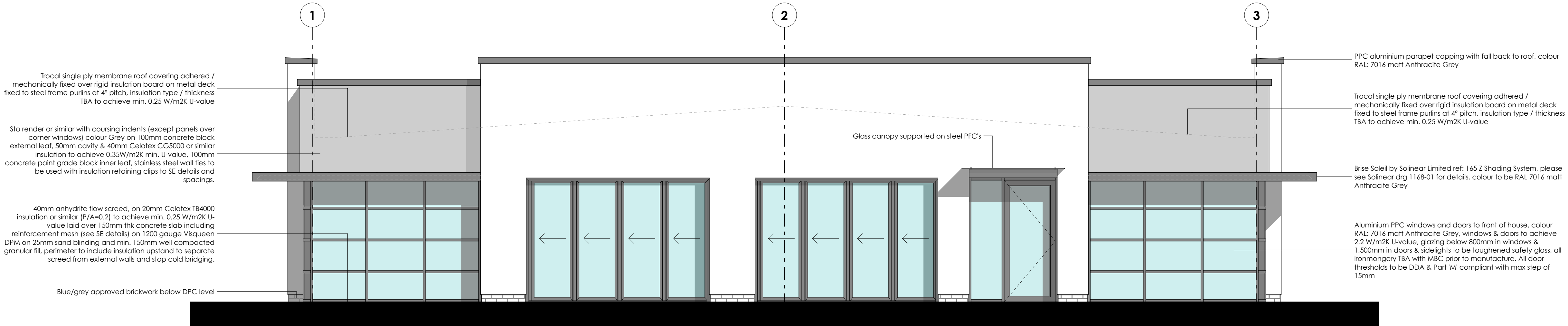
Elevations 1:50
