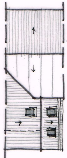
ROOF PLAN 1:200
