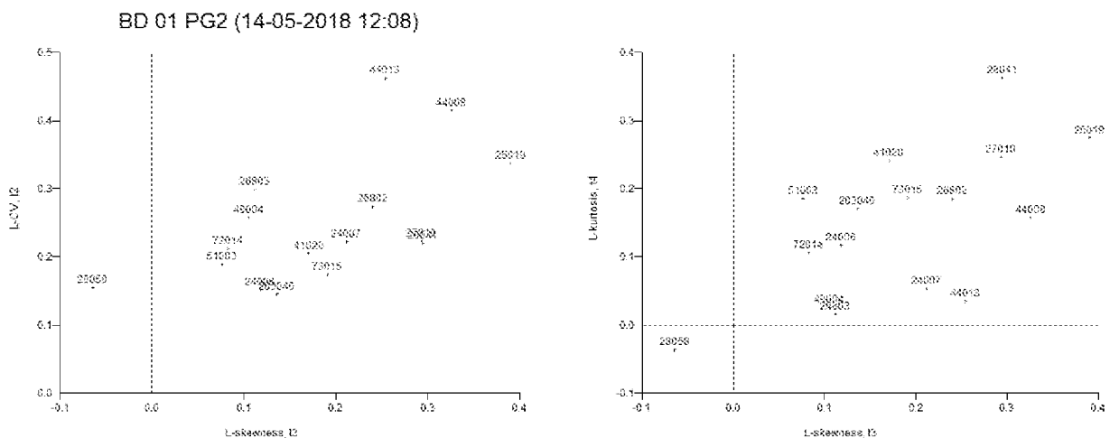
Figure 5: L-moments for final pooling group at site BD_01
