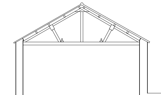
Existing Section 1 1:100
