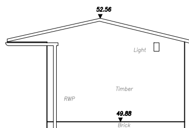
Existing Elevation 7 1:100
