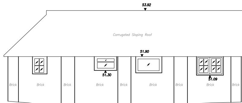
Existing Elevation 9 1:100
