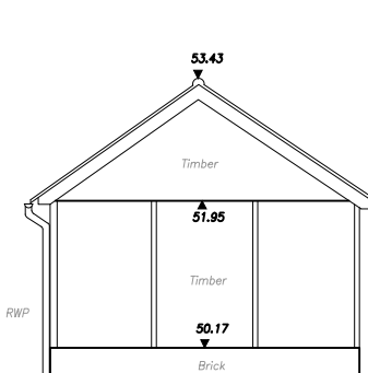
Existing Elevation 11 1:100
