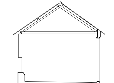
Existing Section 2 1:100
