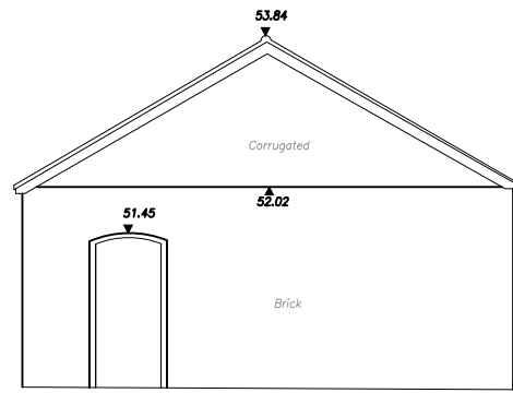
Existing Elevation 1 1:100
