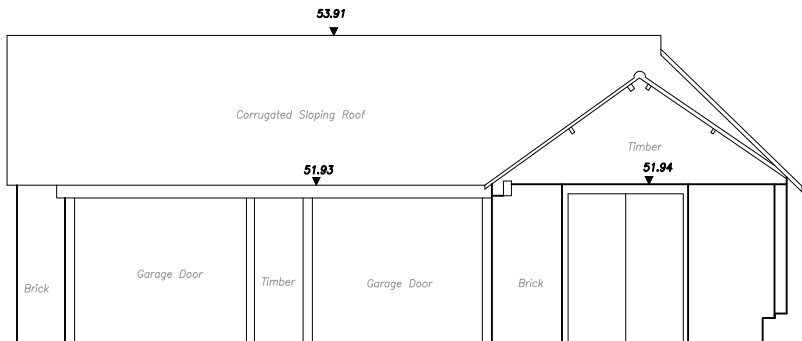
Existing Elevation 11 1:100
