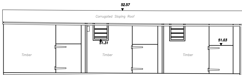
Existing Elevation 5 1:100
