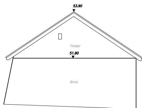
Existing Elevation 14 1:100
