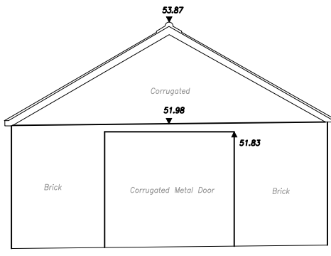
Existing Elevation 3 1:100
