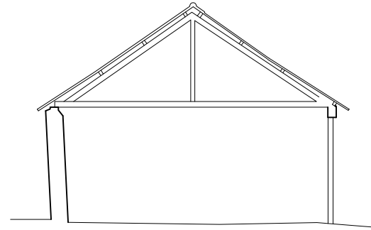
Existing Section 3 1:100
