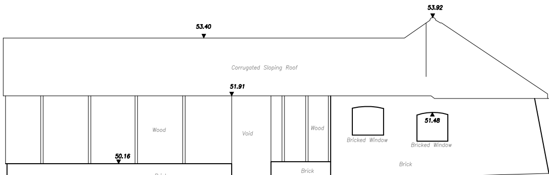
Existing Elevation 10 1:100
