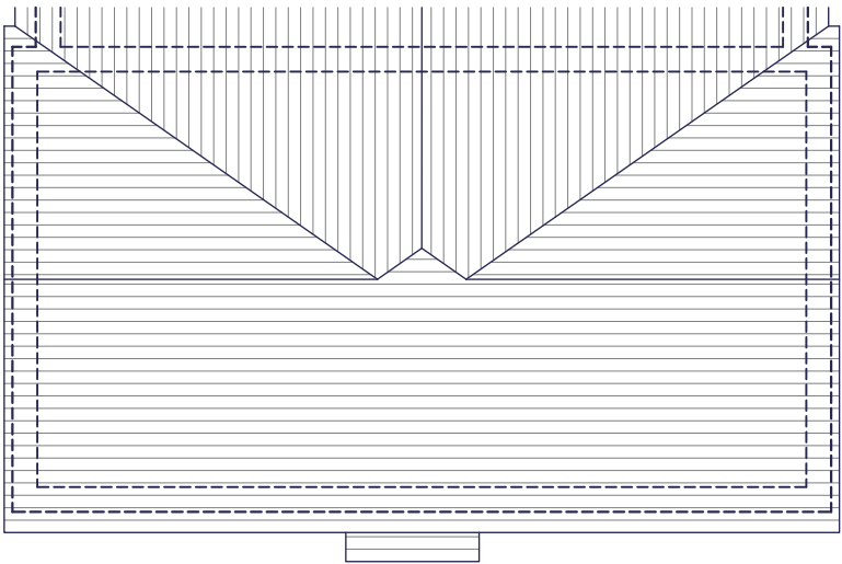
ROOF PLAN
