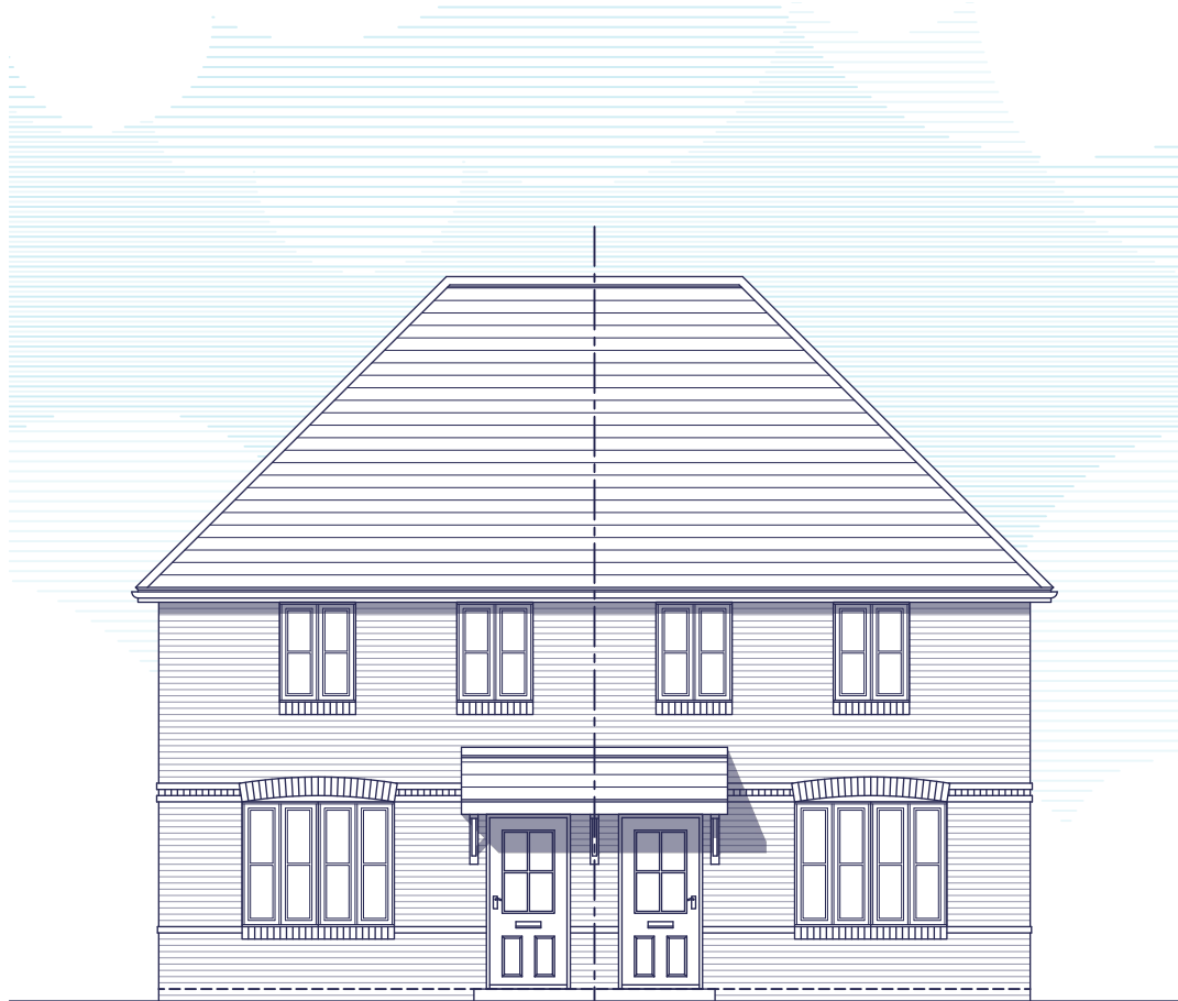
FRONT ELEVATION
