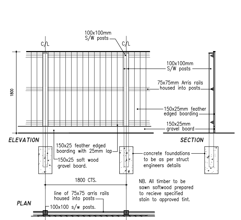
CLOSEBOARD FENCE DETAIL 1:50
