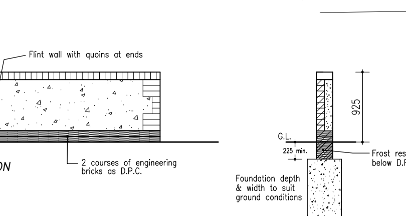
FLINT WALL DETAIL 1:50
