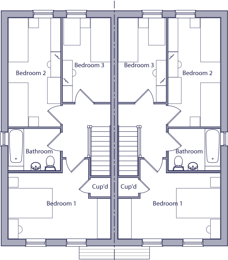
FIRST FLOOR PLAN AS OPP
