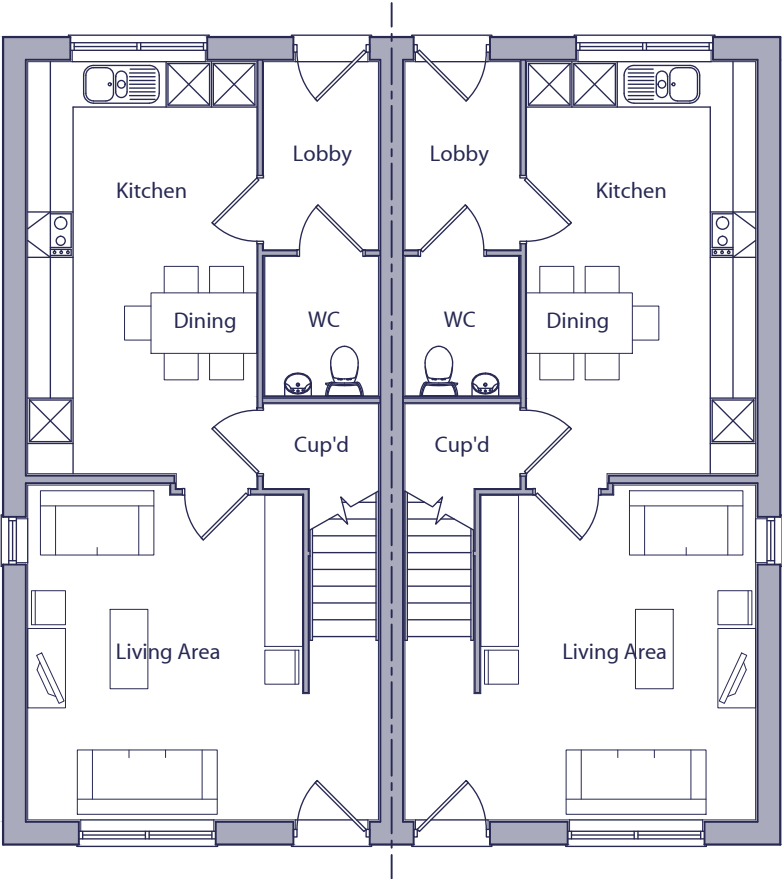
GROUND FLOOR PLAN AS OPP
