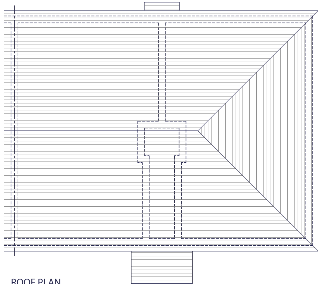
ROOF PLAN
