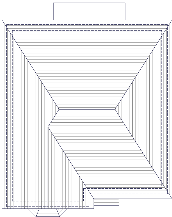
ROOF PLAN
