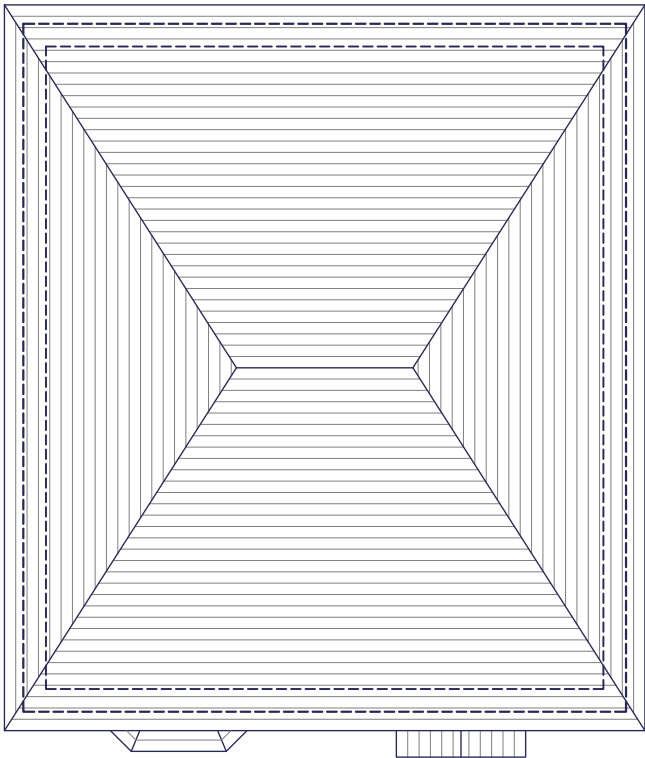
ROOF PLAN
