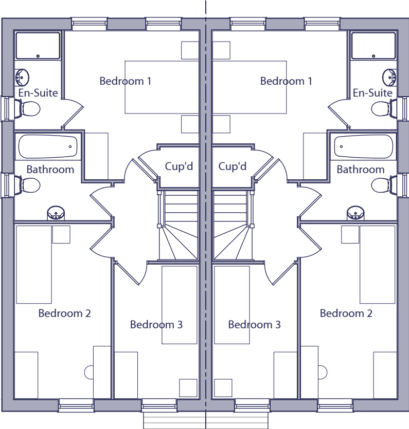
FIRST FLOOR PLAN AS OPP
