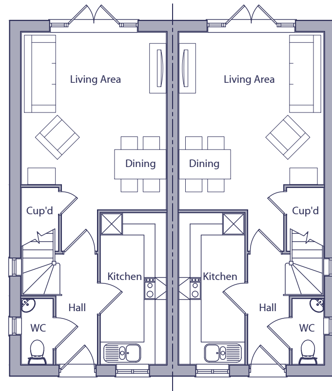
GROUND FLOOR PLAN AS OPP
