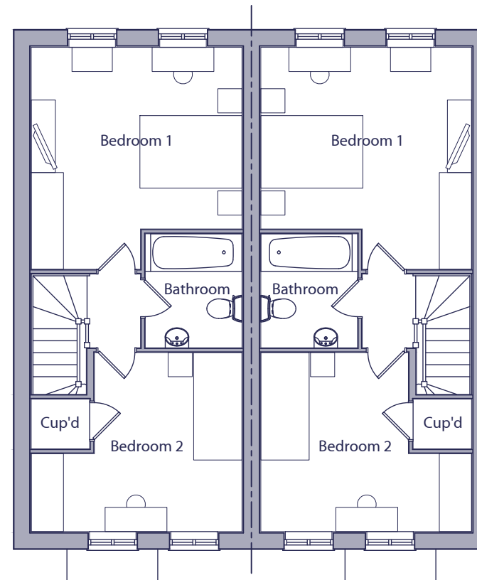
FIRST FLOOR PLAN AS OPP
