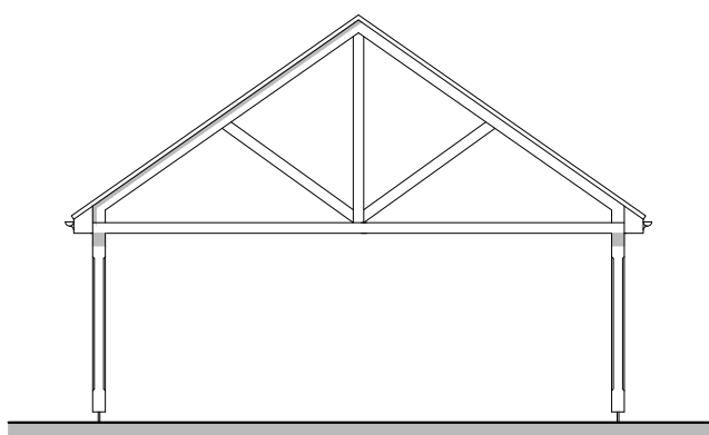
Side Elevations
