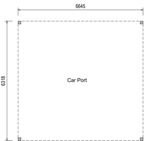
Ground Floor Plan Plots 117/118, 154/155, 473/474, 478/479 & 523/524
