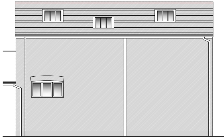
Pr. East Elevation (rear) 1:100 @ A3
