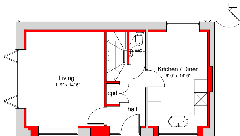
Pr. Ground floor plan 1:100 @ A3
