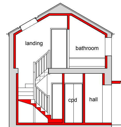
Typical Section 1:100 @ A3
