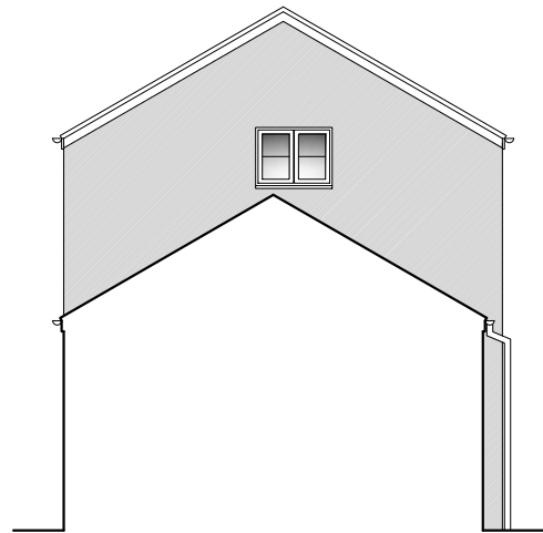
Pr. South Elevation (side) 1:100 @ A3
