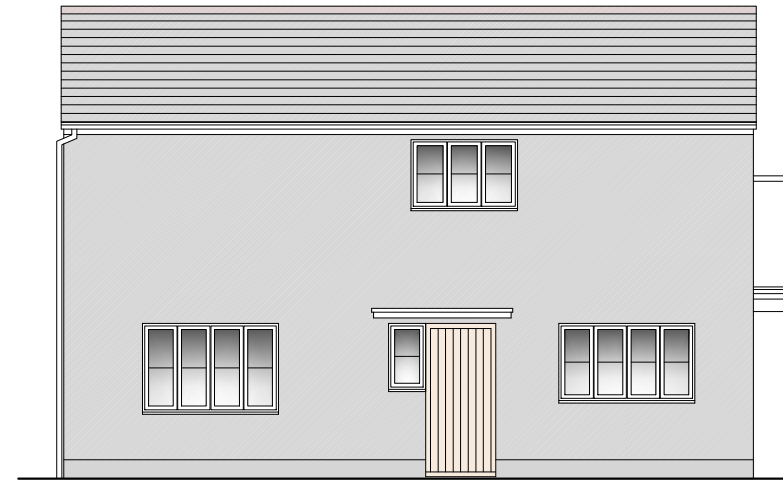
Pr. West Elevation (front) 1:100 @ A3
