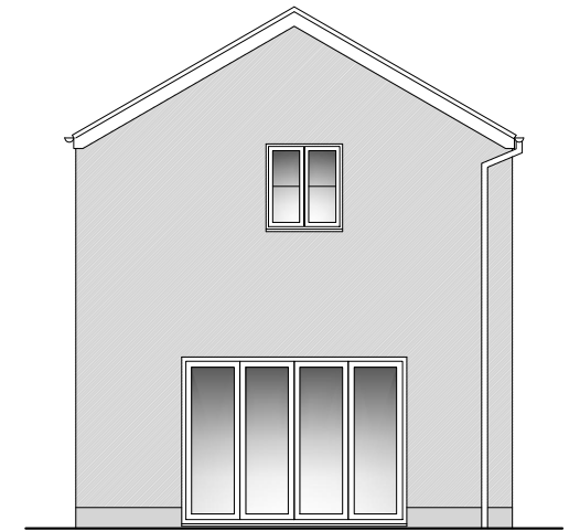
Pr. North Elevation (side) 1:100 @ A3
