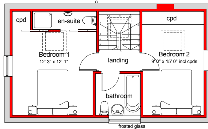
Pr. First floor plan 1:100 @ A3
