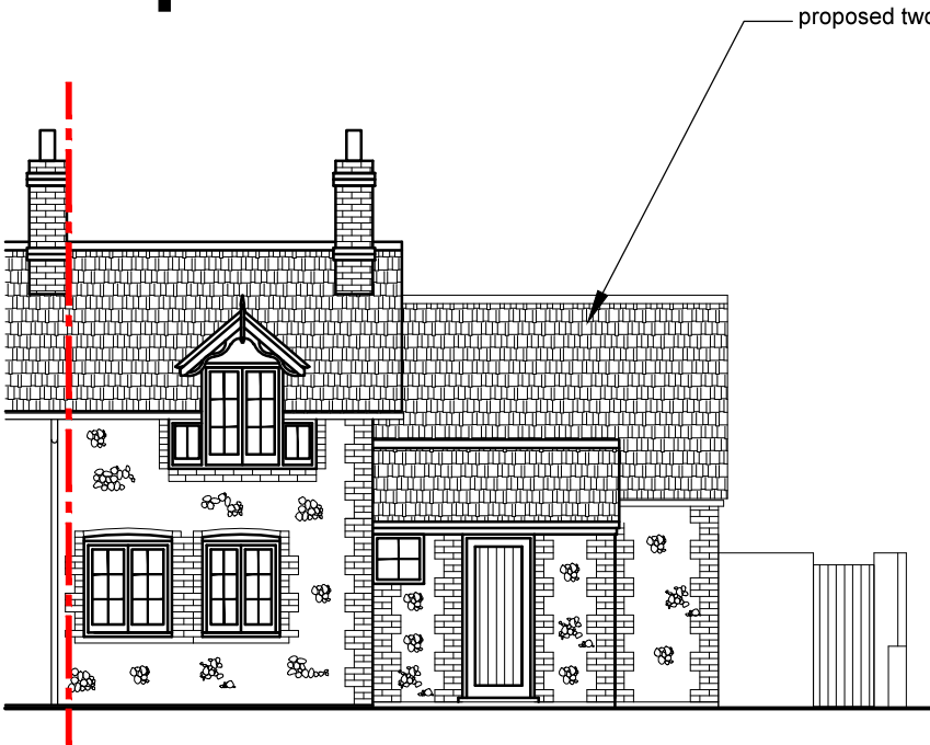
East Elevation 1:100@A3
