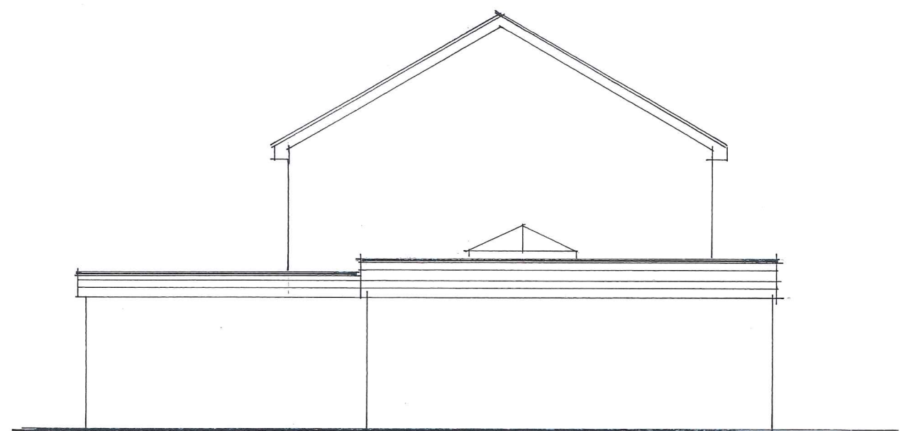
SIDE ELEVATION WEST PROPOSED 1-100.
