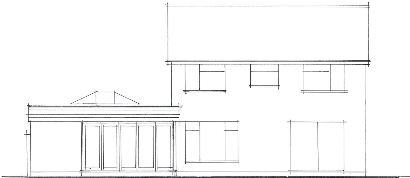
REAR ELEVATION SOUTH PROPOSED 1-100.
