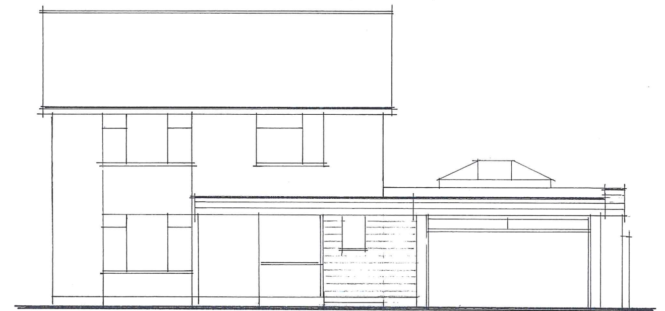
FRONT ELEVATION NORTH PROPOSED 1-100
