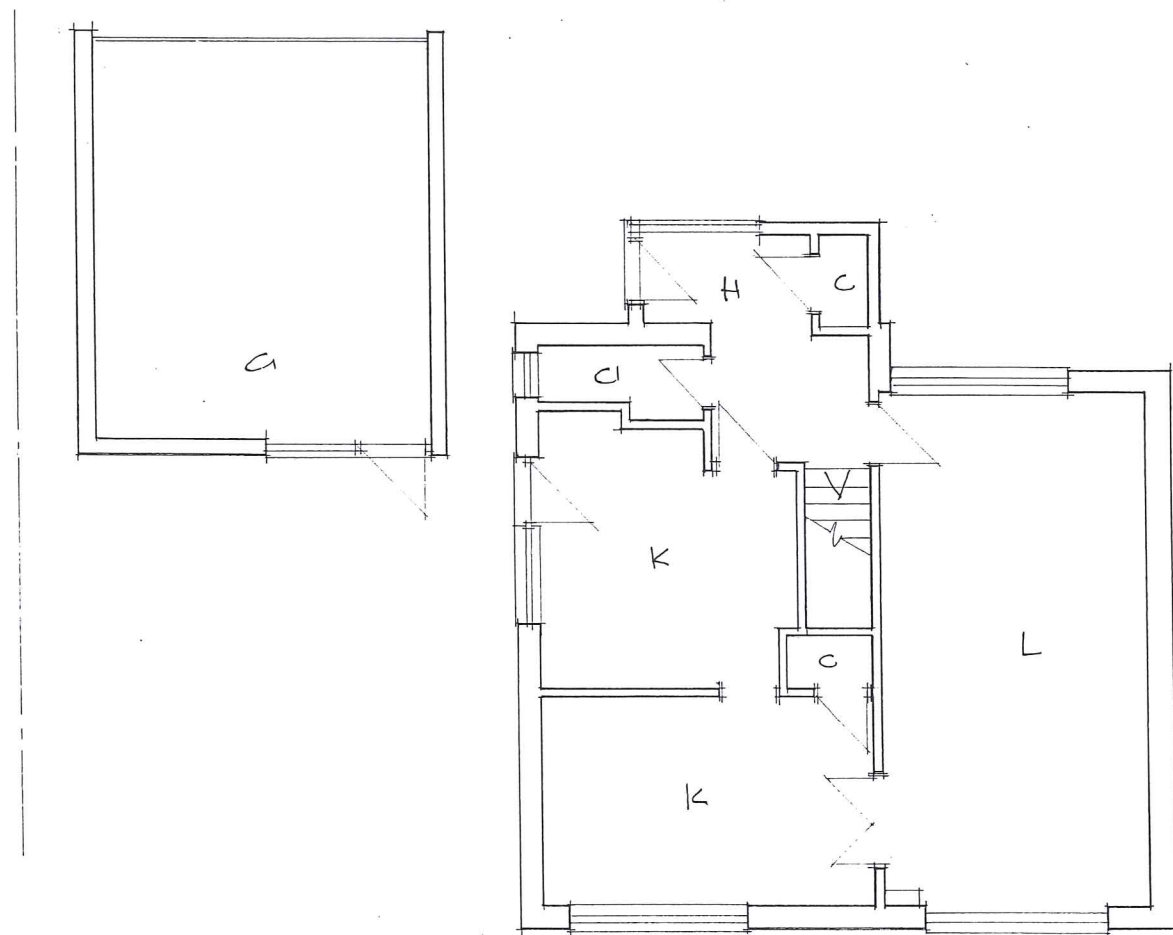
GROUND FLOOR PLAN EXISTING 1-100
