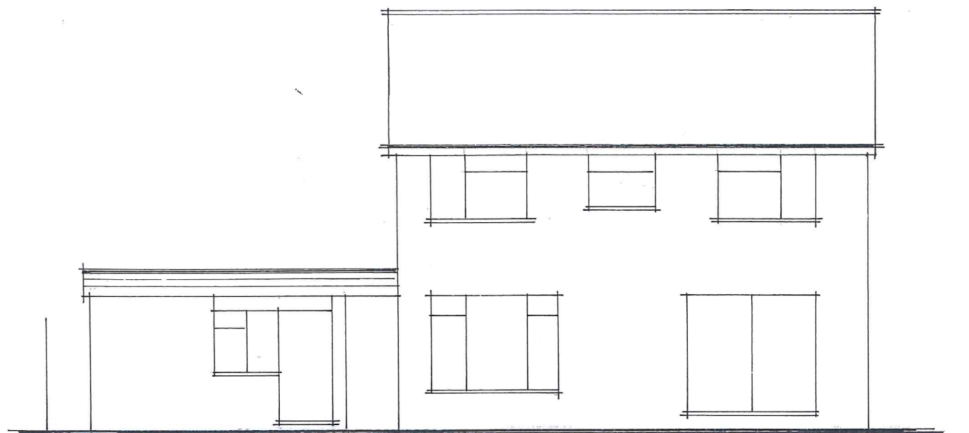
REAR ELEVATION SOUTH EXISTING. 1-100
