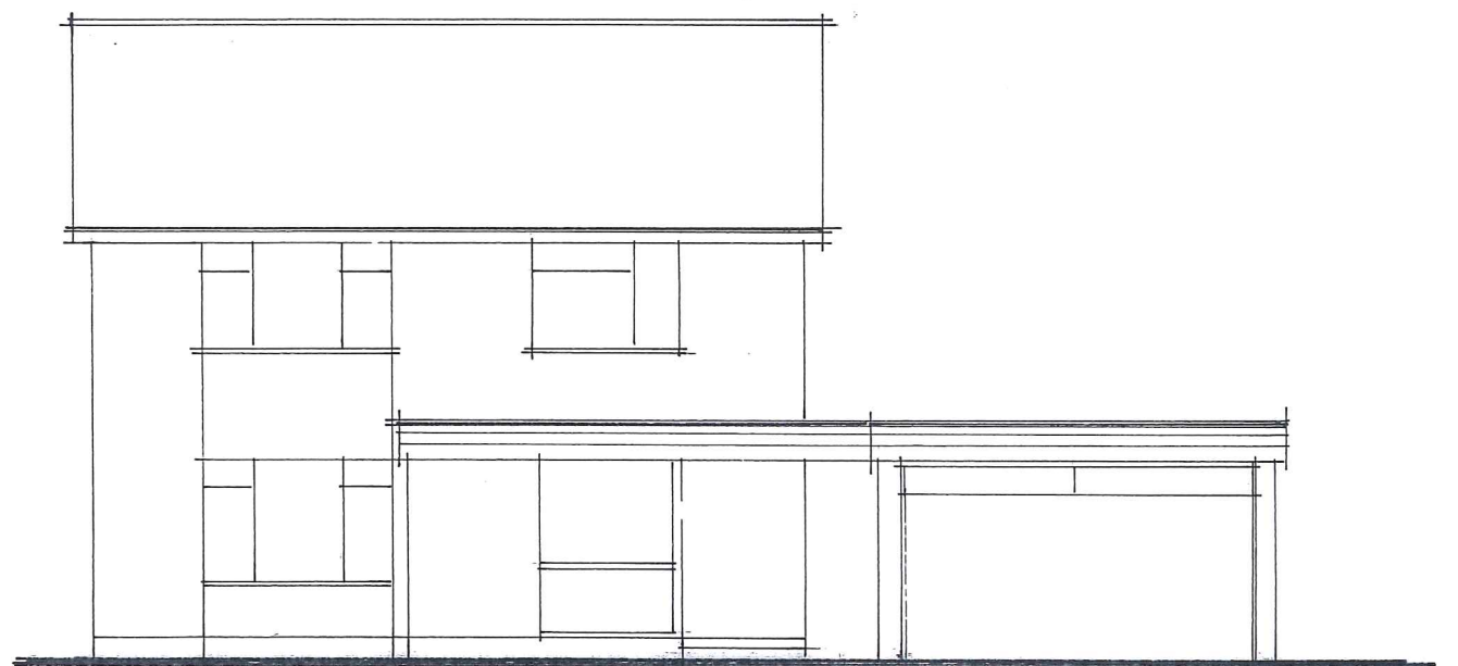
FRONT ELEVATION NORTH EXISTING. 1-100
