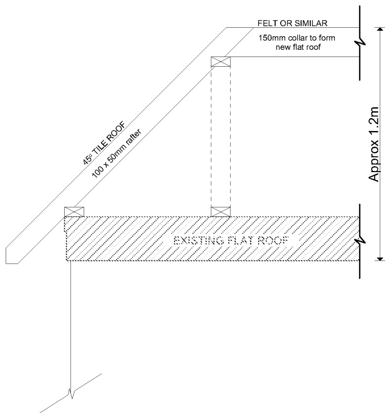
Sketch cross section showing the proposed roof
