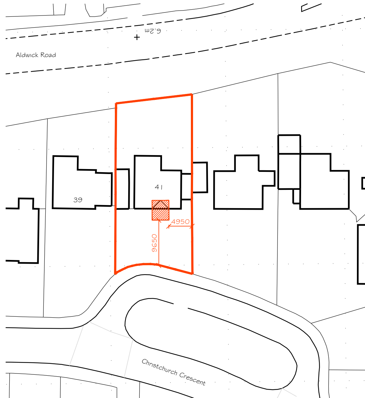
Block Plan
