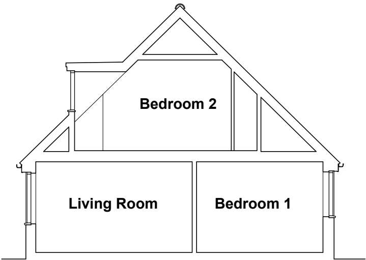
EXISTING SECTION A-A @ 1:100
