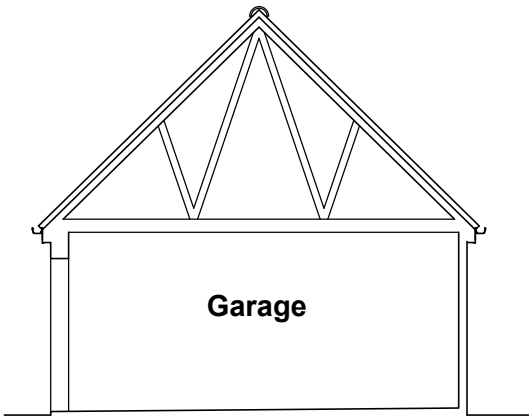
EXISTING SECTION B-B @ 1:100
