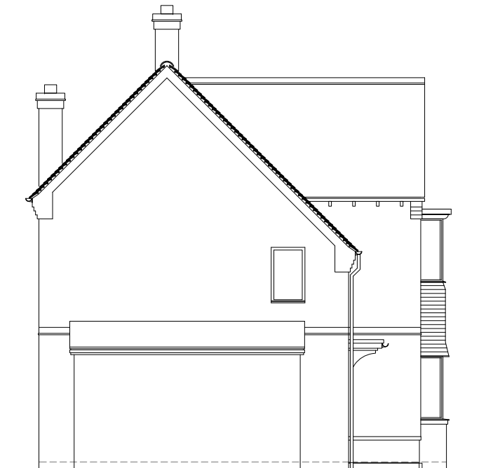
SOUTH EAST ELEVATION
