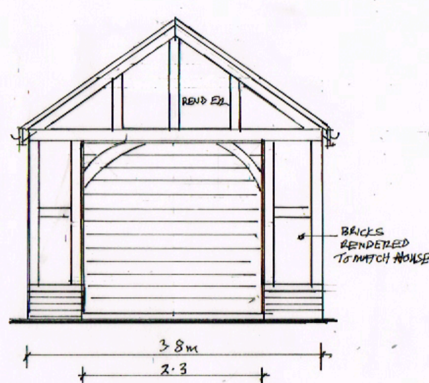
FRONT (NORTH)
