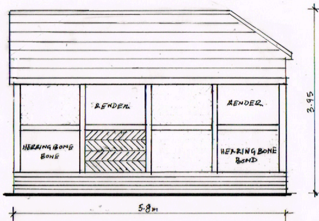
SIDE (WEST)
