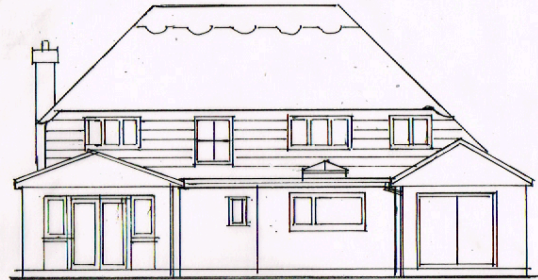
REAR (EAST)
