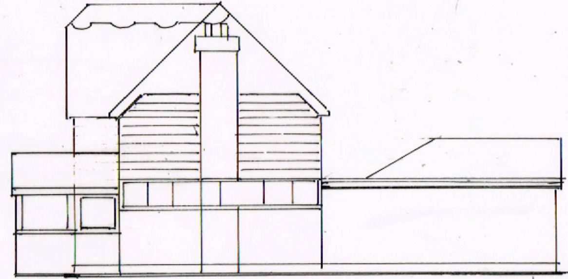
SIDE (SOUTH)
