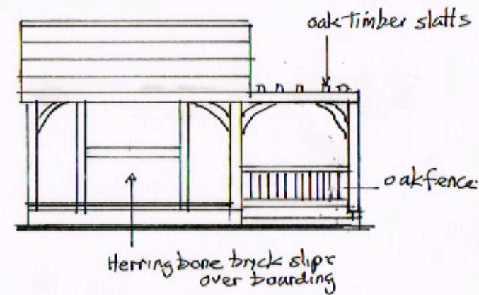
REAR (EAST)
