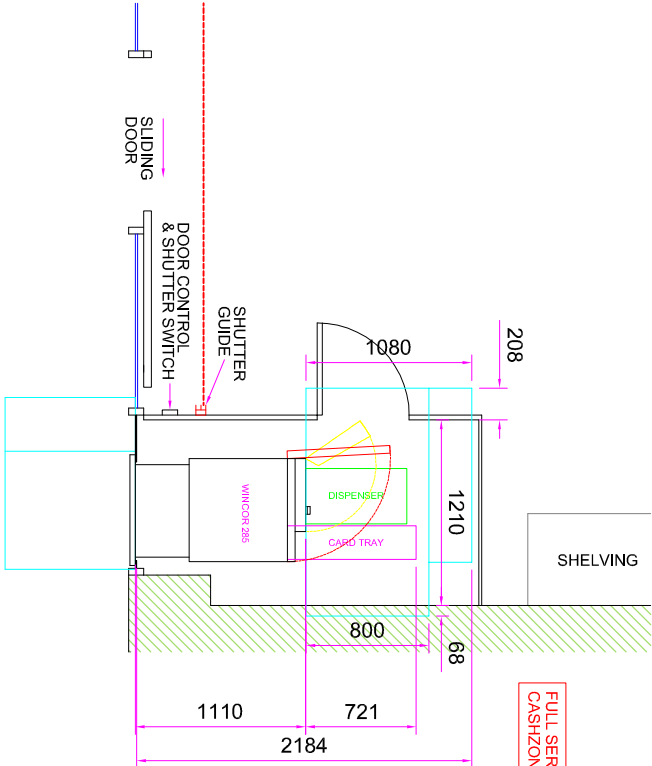
PROPOSED (PART) PLAN
