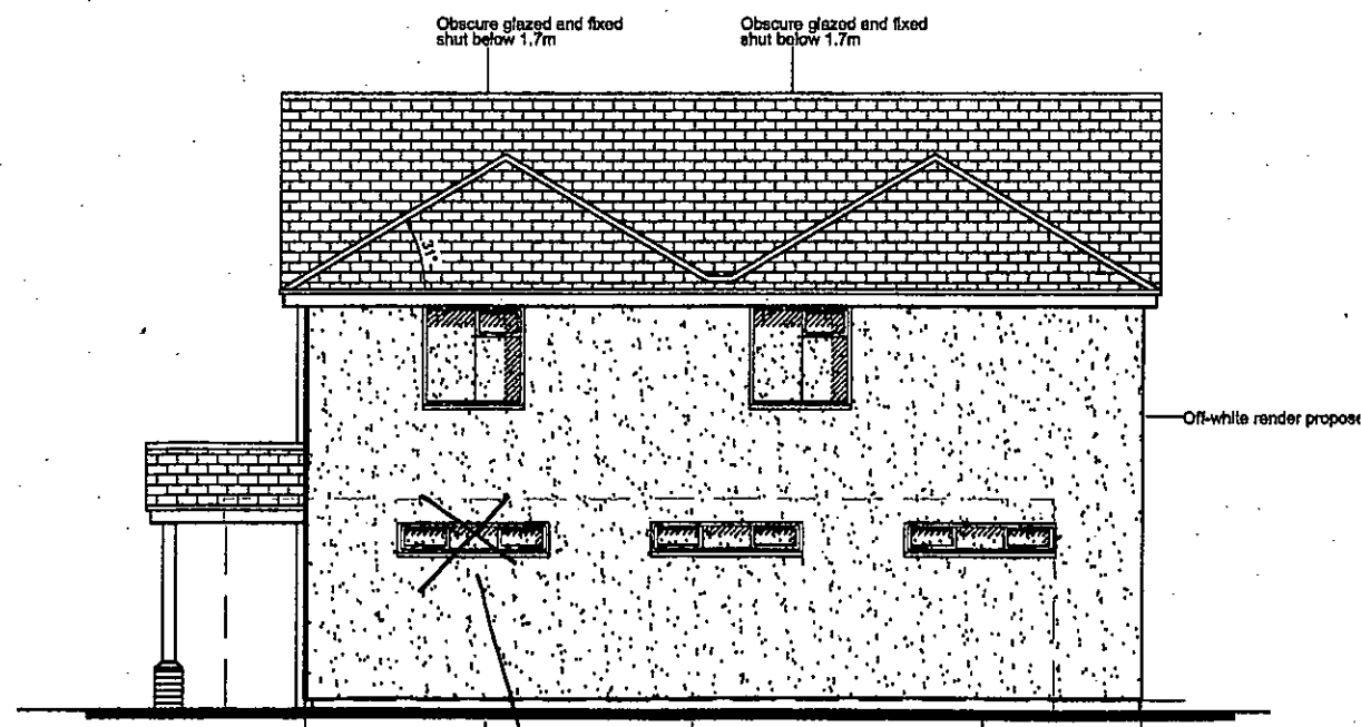
RIGHT (WEST)
