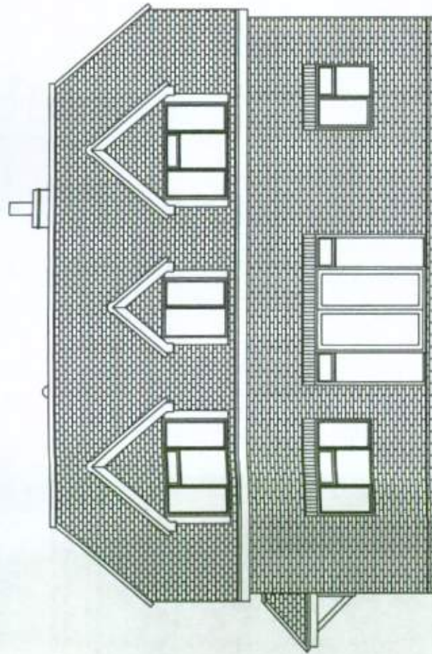
NEW NORTH ELEVATION
