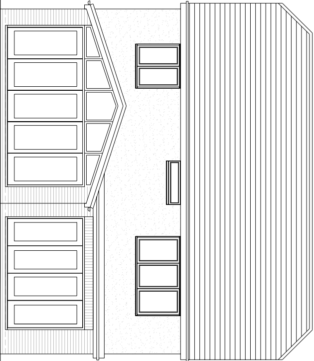
Rear Elevation
