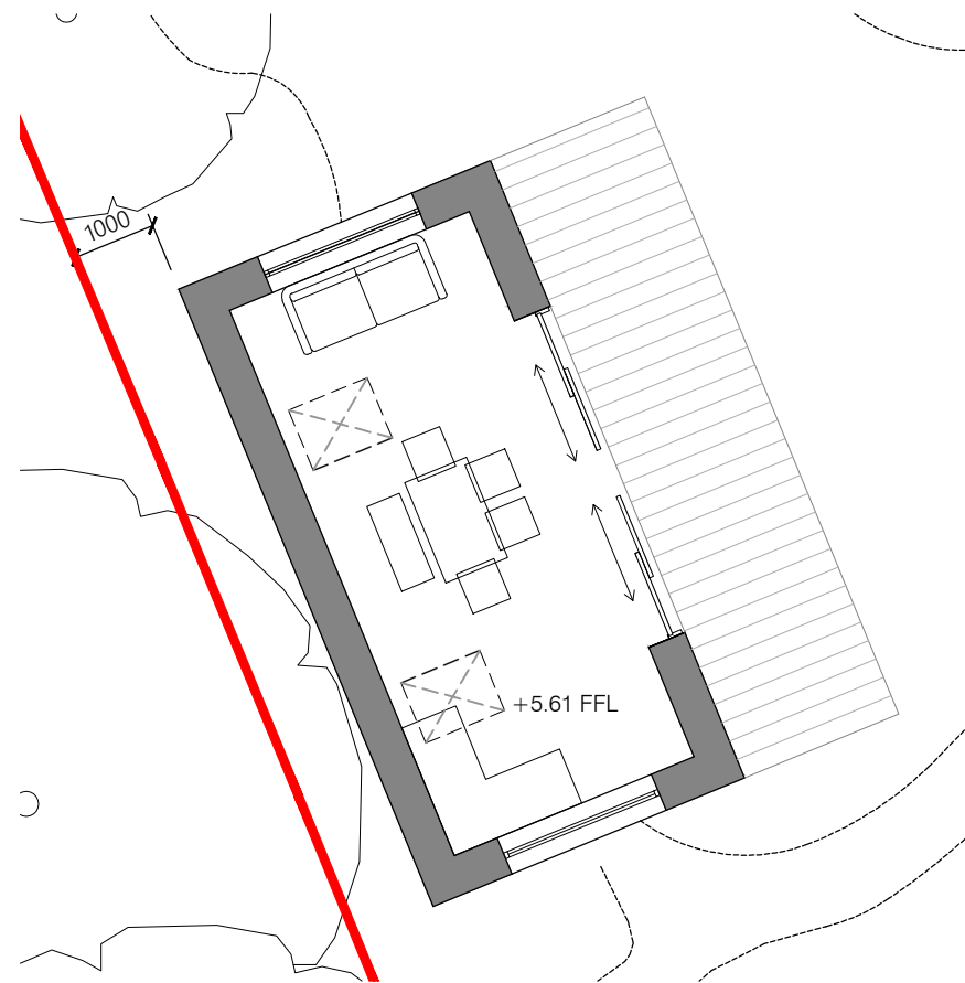
Proposed Plan
