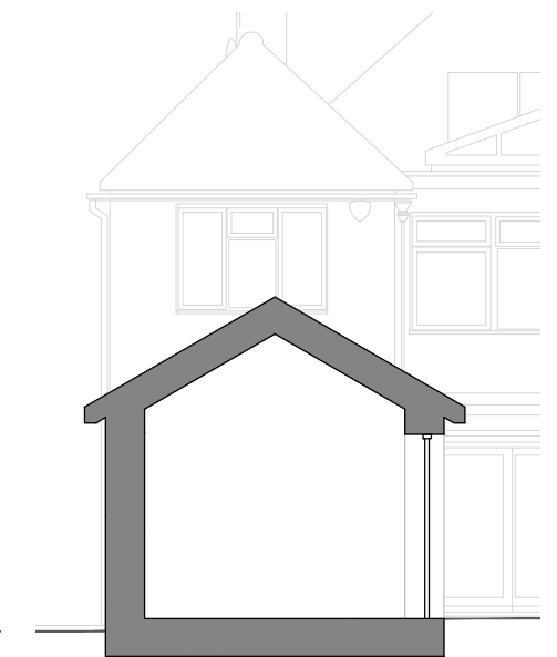
Proposed Section
