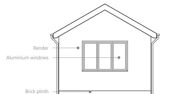
Proposed North Elevation
