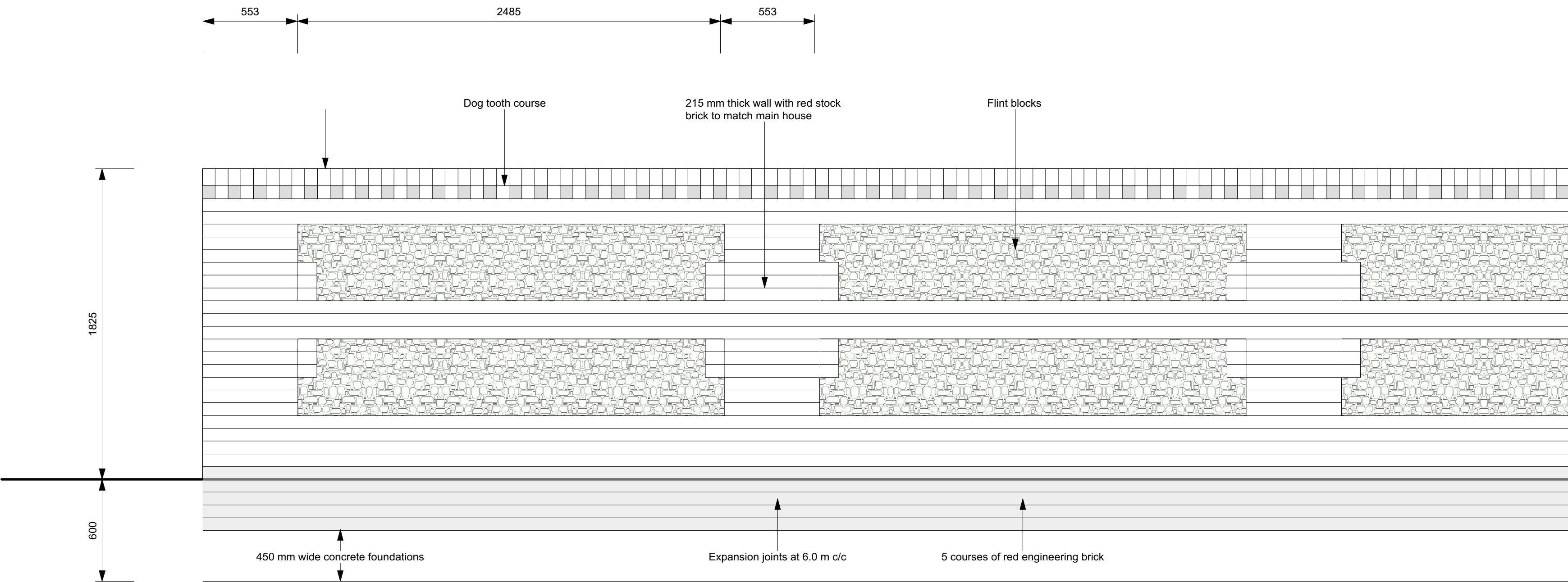
Detail Elevation
