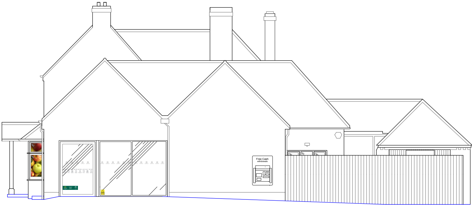
SIDE ELEVATION
