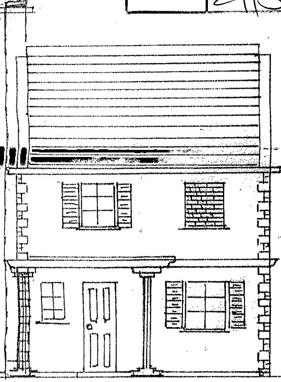
South Elevation
