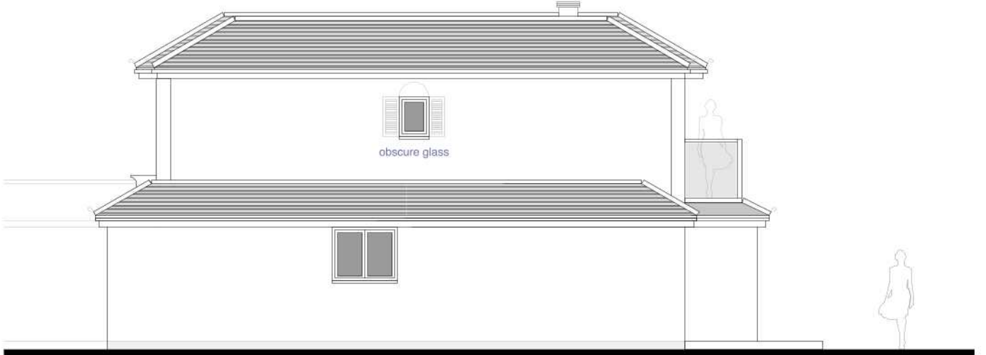
(GARAGE BEYOND NOT SHOWN) Proposed Side Elevation at 1:100 scale WEST
