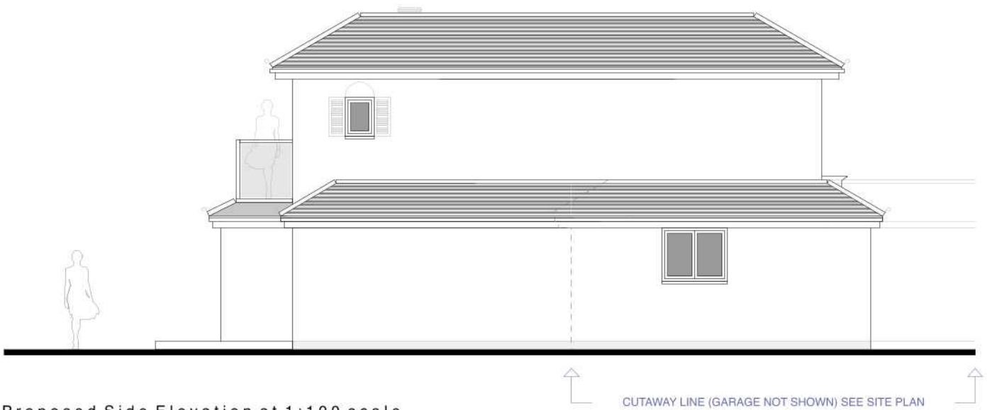
Proposed Side Elevation at 1:100 scale EAST
