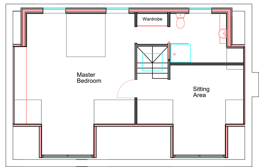
PROPOSED ATTIC PLAN
