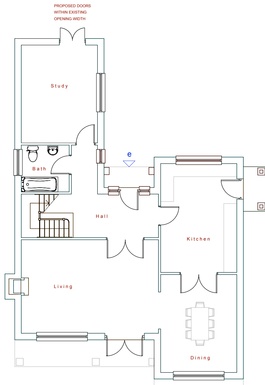
Proposed Ground Floor Plan at 1:100 scale
