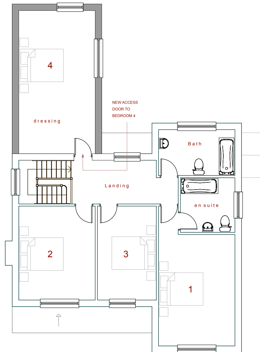
Proposed First Floor Plan at 1:100 scale
