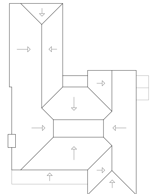
Proposed Roof Plan at 1:100 scale
