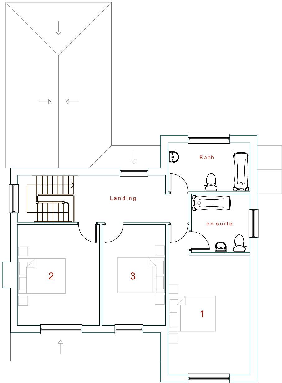
Existing First Floor Plan at 1:100 scale
