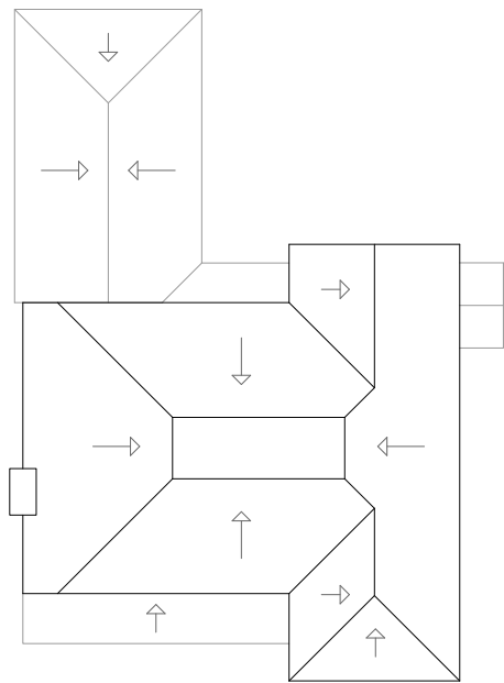
Existing Roof Plan at 1:200 scale
