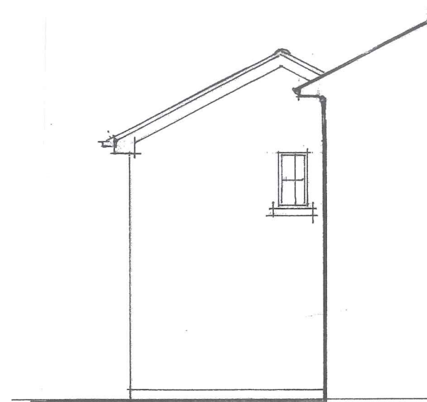
SIDE EL. (WEST) H100 EXTENSION
