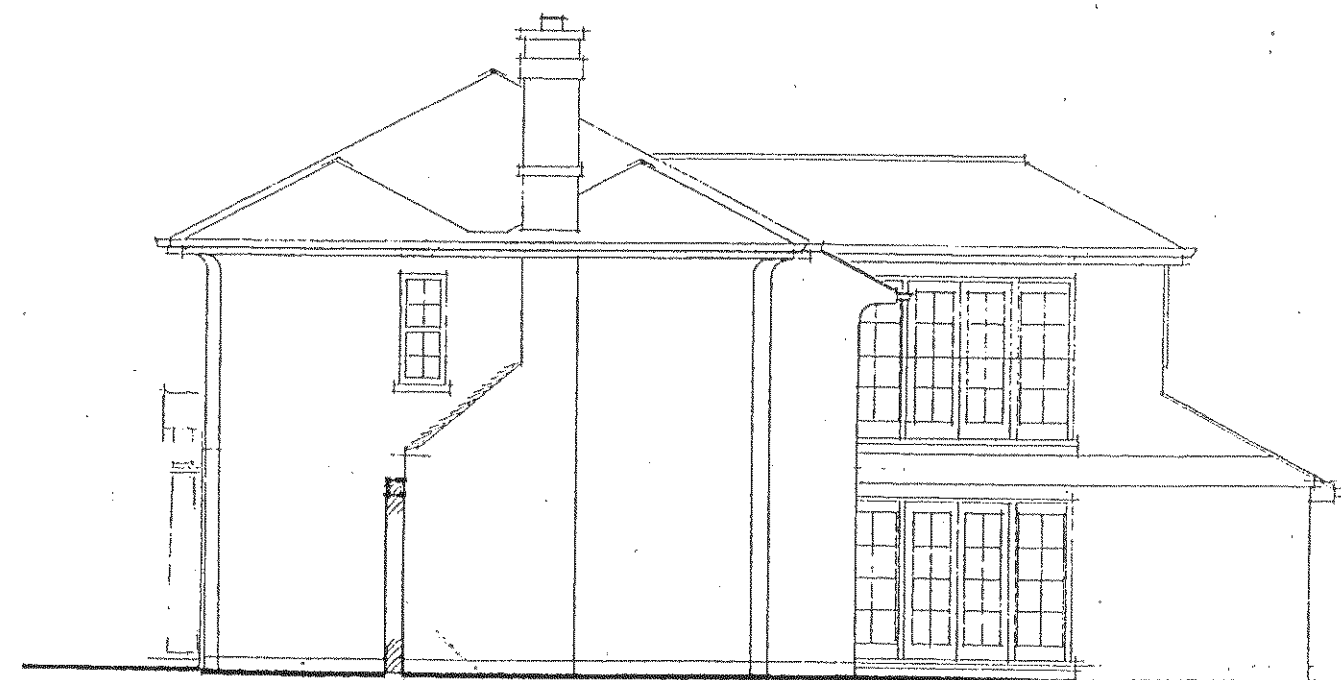
SIDE ELEVATION - EAST 1-100
