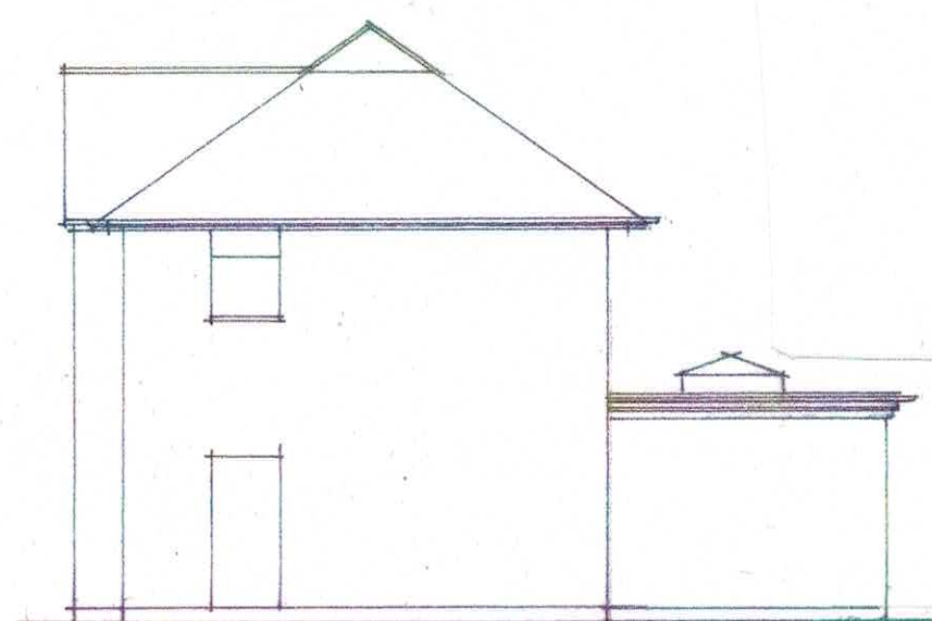
SIDE ELEVATION WEST 1:100
